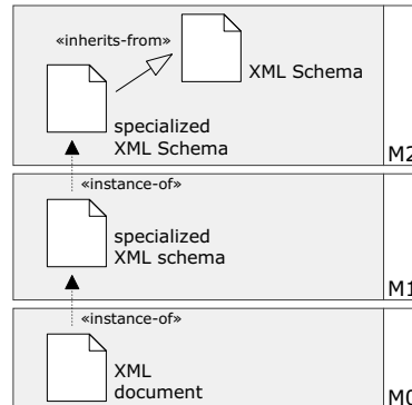
Fig. 4. Specialized XML Schema Approach
