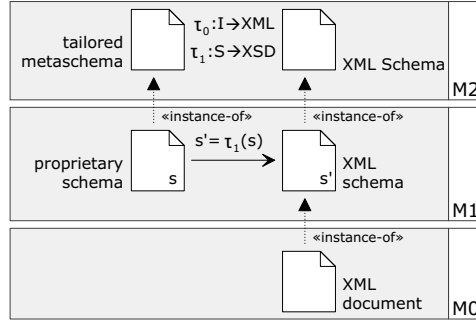
Fig. 2. Side by Side Approach
