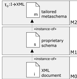
Fig. 1. Proprietary Schema Approach
